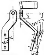
Figs. 3007-3009. Lubricator Bracket.
